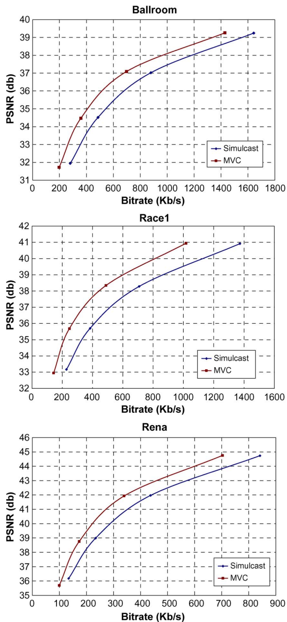
Fig. 5. Sample coding results for several MVC test sequences, including Ballroom, Race1, and Rena sequences, according to common test conditions [48].
