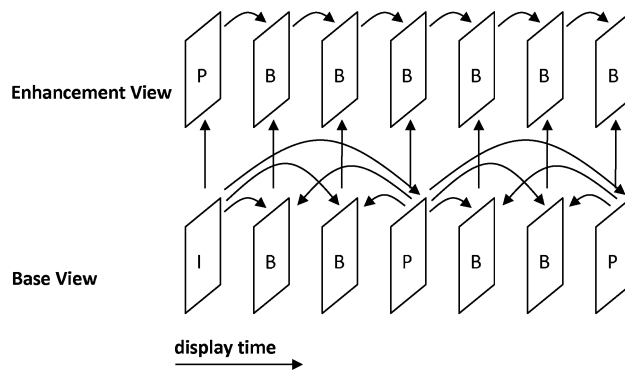
Fig. 1. Illustration of inter-view prediction in H.262/MPEG-2.
